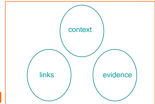
Island model
